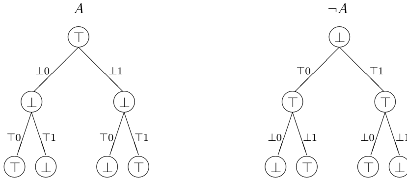
Figure 5: Negation
