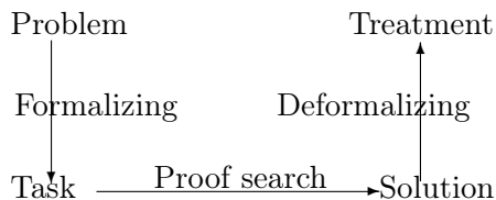
Fig. 1. Solving process
